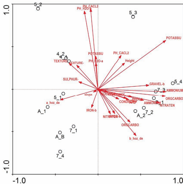
FIG 4 - Environmental redundancy analysis bi-plot of all species, all environmental variables and sites where soil was collected (14 sites). Length of arrow is proportional to strength of correlation between environmental variables and axes (major floristic gradients). Note: Site A_1 is PD_1, Site A_2 is PD_2 and Site A_B is PD-PS transition.
